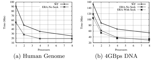
Figure 12: Shared-memory, shared-disk; strong scalability; 16GB RAM divided equally among cores
