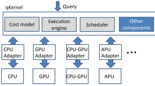
Figure 2: The kernel-adapter design of OmniDB.
