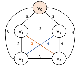
Figure 8: Undirected Graph G
