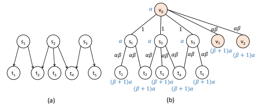
Figure 5: Illustration of Proof of Lemma 5
