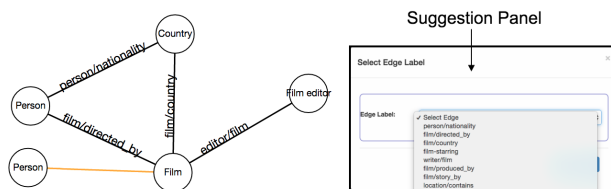
Figure 5: Adding Edge in Active Mode
