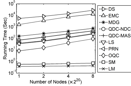
Figure 11: Running time on the synthetic networks
