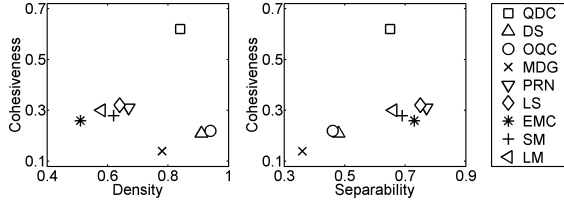
Figure 6: Goodness metrics on the LJ network
