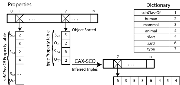
Figure 1: Sort-Merge-Join Inference: CAX-SCO.
