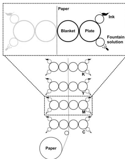
Figure 1: Key elements in a printing press.
