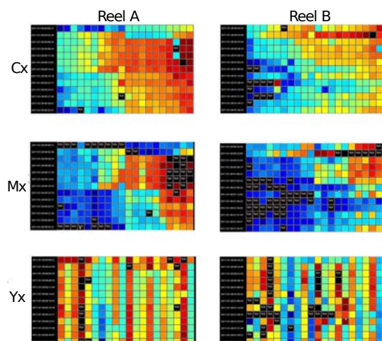
Figure 7: Matrices of miss-registration degree for cyan, magenta, and yellow inks measured by the virtual sensor.
