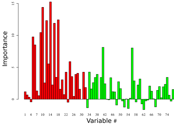
Figure 5: Variable importance when modeling black ink density variation. Full range press velocity was used.
