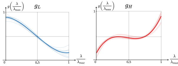
Figure 3: Filters g_L and g_H learned from Elliptic by AMNet.
