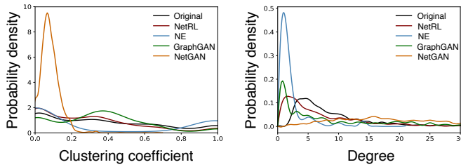
Fig. 4: Clustering coefficient and degree distributions of the original network and denoised networks of Wiki.
