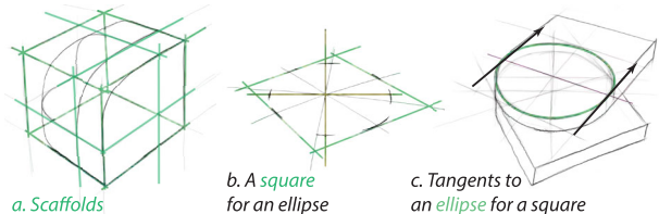
Fig. 3. (a) 3D scaffold for a rounded corner, (b) 2D square scaffold for an ellipse and (c) ellipse scaffold for a square.
