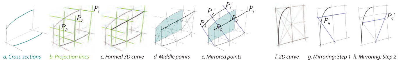
Fig. 4. Cross-section planes and mirroring techniques: (a) two cross sections, (b) points formed by intersection of a set of projection lines, (c) derived 3D crease, (d) and (e) mirroring with respect to cross-section plane by duplicating the rectangles (the mirrored crease is obtained by drawing a line through mirrored points); (f) 2D curve to mirror, its scaffold, (g) finding the point to mirror as the intersection of the line perpendicular (in space) to the mirroring axis and the diagonal of the formed rectangle, (h) the mirrored point construction as a projection of the reference point on the mirrored diagonal. A mirrored curve is obtained by defining multiple such points.
