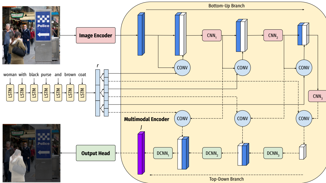
Figure 1. Overview of the proposed model on the task of referring expression segmentation.
