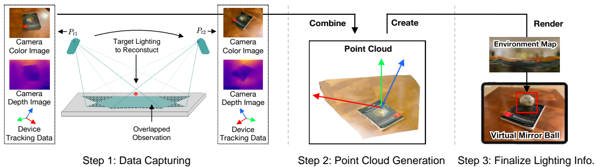
Fig. 2. A simplified workflow of mobile AR lighting reconstruction. In this example, the mobile device starts at position P_{11} and points toward the rendering position on the table specified by the mobile user. Data such as color and depth images, as well as device tracking data, will be captured. The device will further capture more data (e.g., color/depth images from a different viewing direction) at position P_{12} , which naturally overlaps with the data captured at P_{11} . The data is maintained in a fixed-size buffer and will be aggregated to generate a global multi-view point cloud. We will update the point cloud as new data arrives and use it to generate the final environment map for virtual object rendering.
