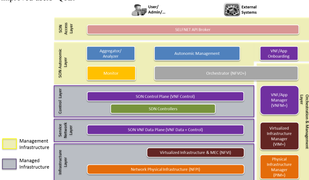
Figure 5-22: Overall Self-Optimized Architecture
