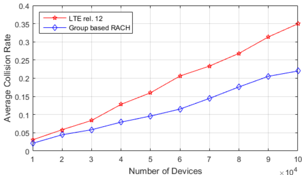
Figure 3-9: Group-based initial access gains in terms of average collision rate decrease [3-1]
