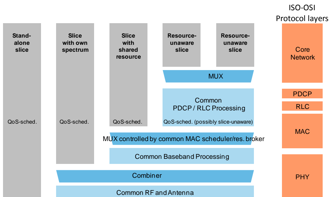
Figure 2-6: Options for slice multiplexing and their relation to the OSI protocol stack [2-26]
