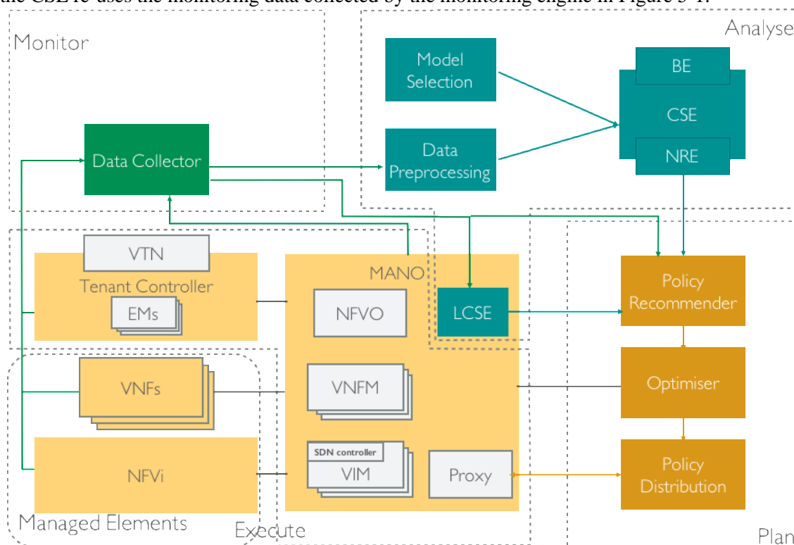
Figure 5-20 CSE in depth functioning architecture mapped to MAPE autonomic loop: Data Sources (Light Orange), Data/Collection (Green), Cognitive Elements (Blue), Policy Engine Elements (Dark Orange).
