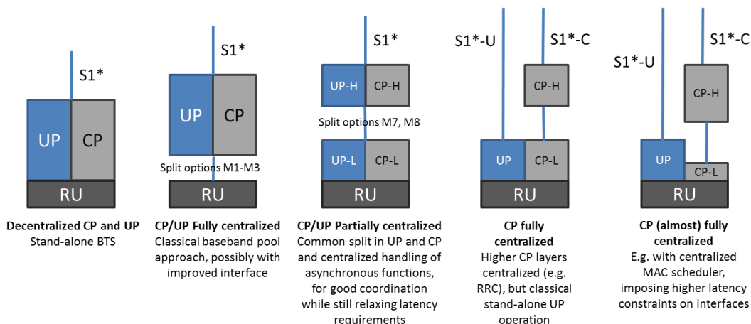
Figure 3-1: Considered UP/CP Split Constellations [3-1][3-2]
