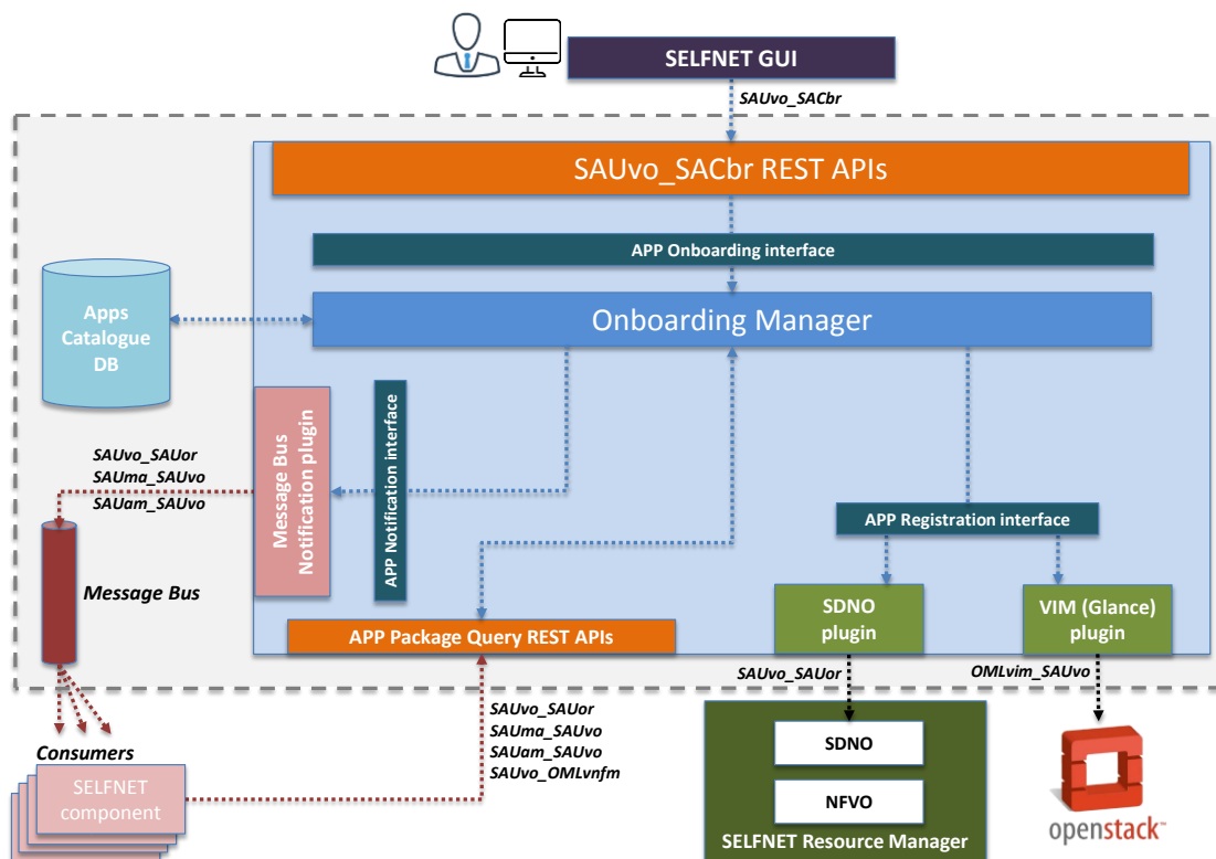
Figure 5-14: VNFs Onboarding Service and Plug-ins
