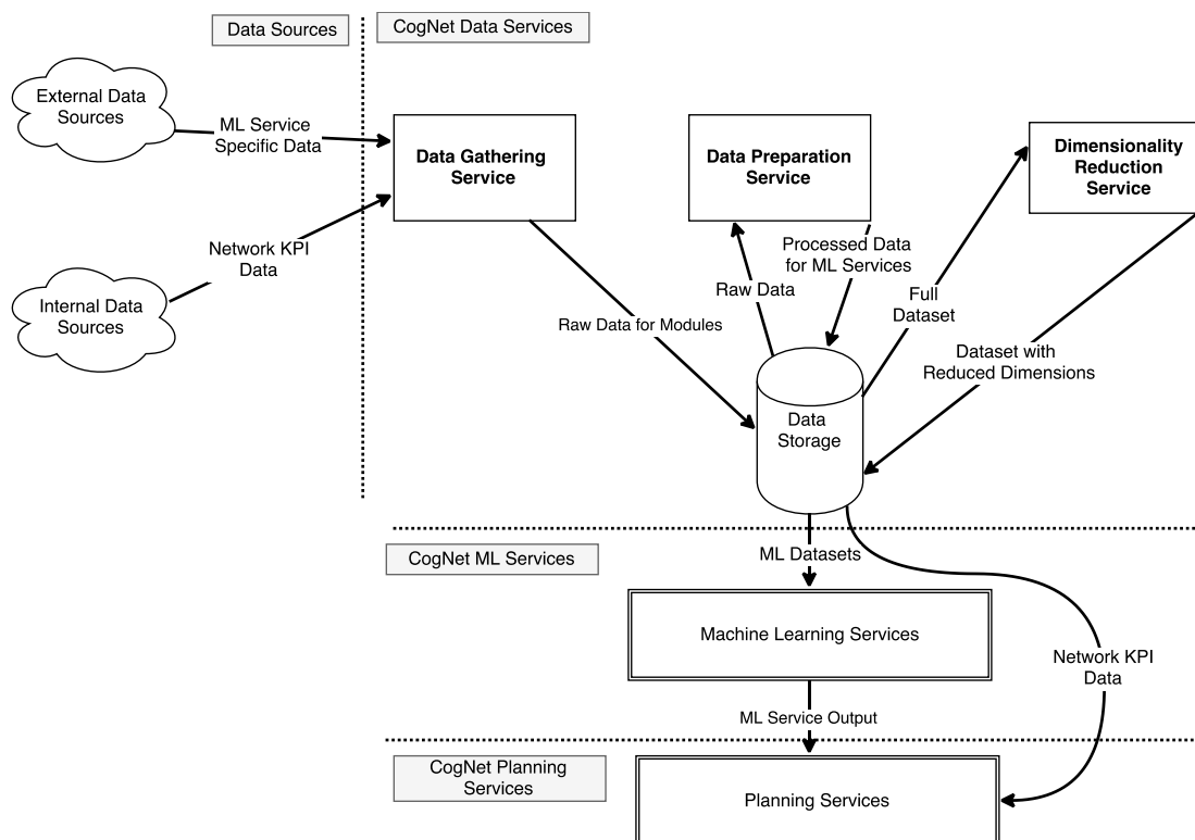
Figure 5-13: Data Services Interface with Input and Output of Each Service.
