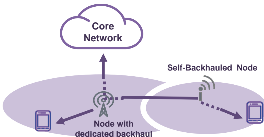
Figure 3-13: Concept of Self-backhauling
