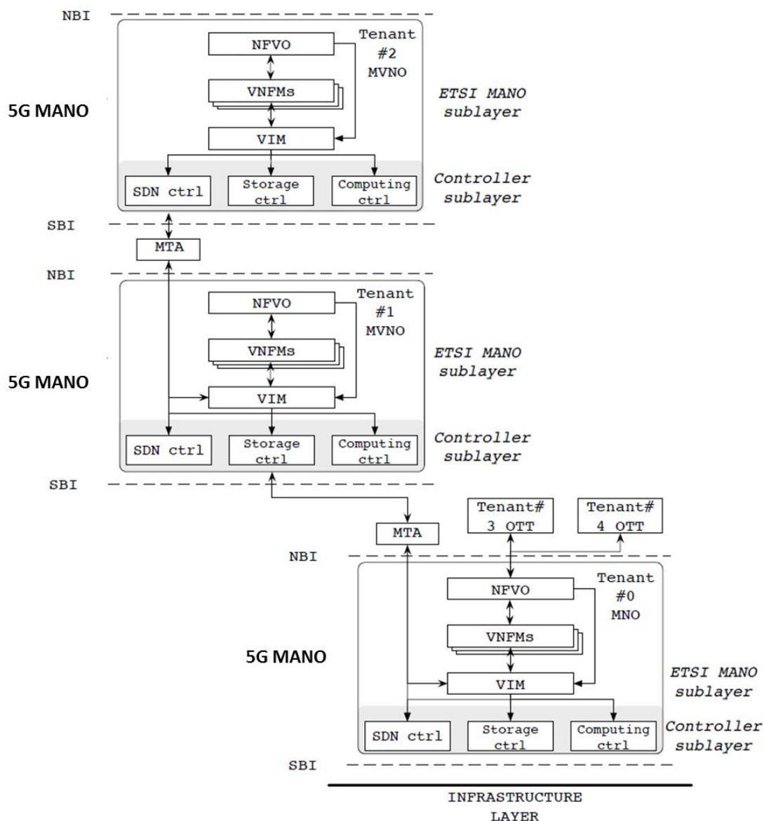
Figure 2-12: Recursive architecture [2-31]
