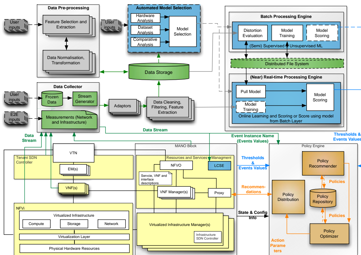
Figure 5-21 CSE Operational Architecture.
