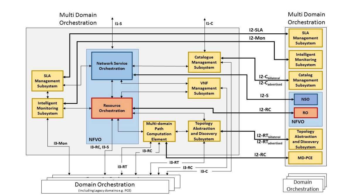
Figure 5-17: Implementation Design Architecture for multi-domain orchestration
