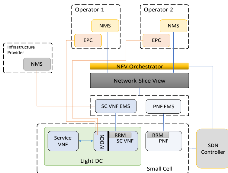
Figure 5-9. Support for RAN sharing through Edge Cloud infrastructure
