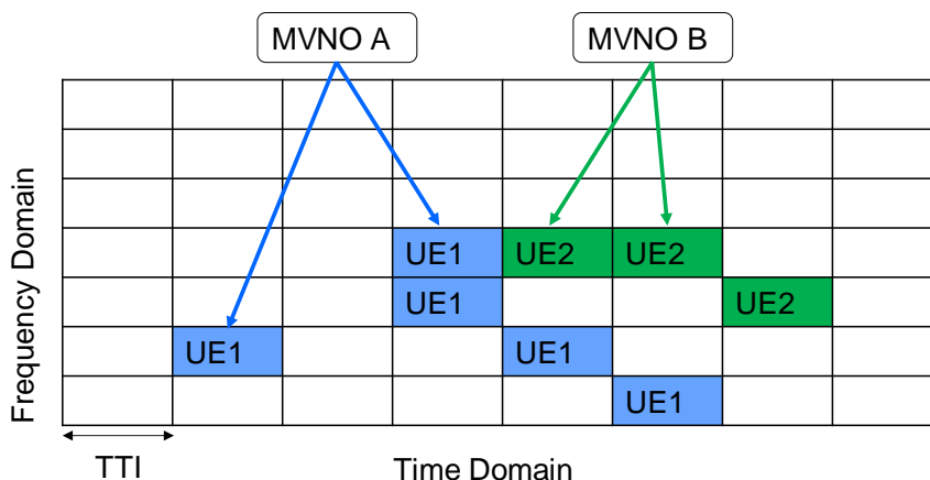
Figure 5-3 RAN sharing
