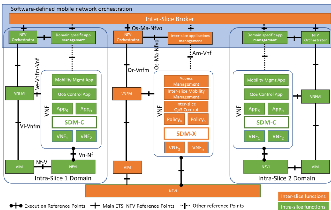
Figure 2-10: Inter- and intra-slice MANO framework [2-29]
