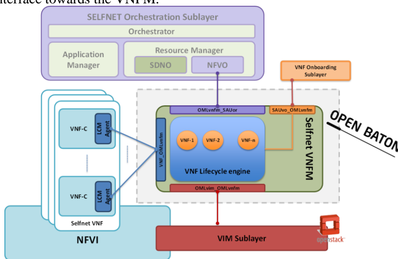
Figure 5-15: SELFNET VNFs Lifecycle Management
