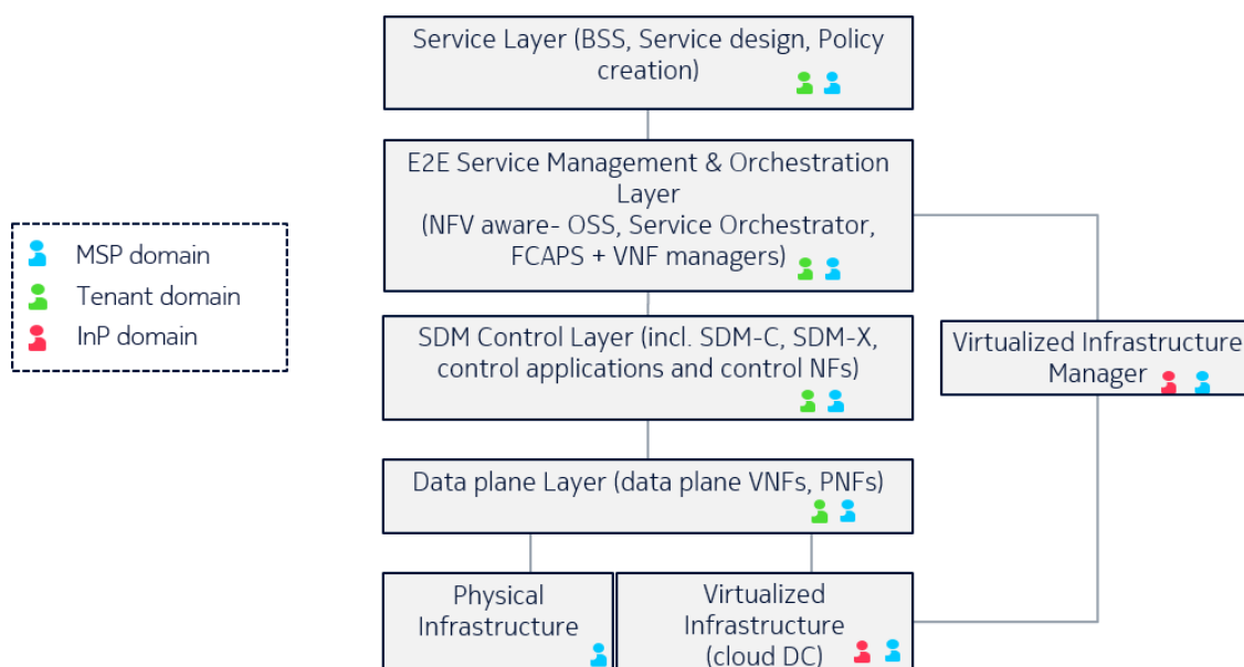
Figure 2-13: Possible domain ownerships of main functional blocks using the layers introduced before [2-26]
