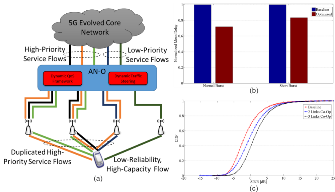
Figure 3-11: Dynamic Traffic Steering framework (a), delay gains (b) and reliability increase in terms of SINR gains (c).
