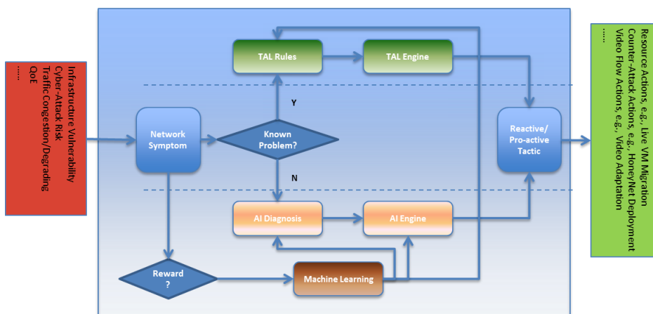
Figure 5-23: Autonomic Network Management Framework: SON Engine
