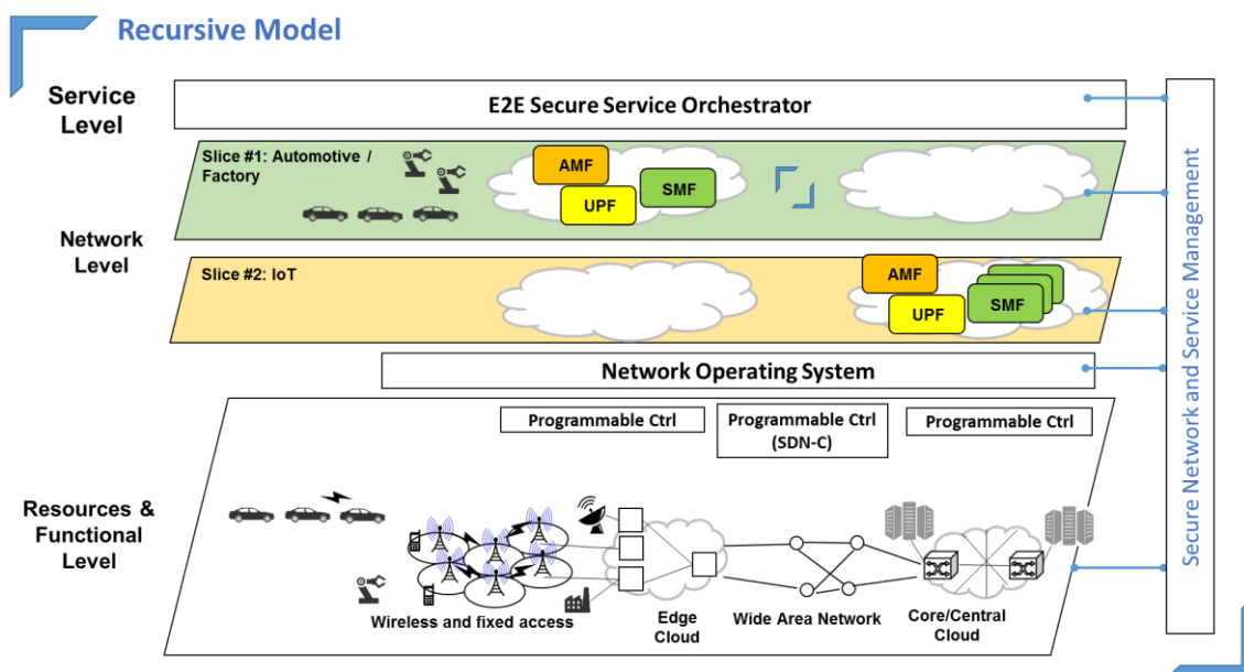
Figure 2-1: Overall Architecture
