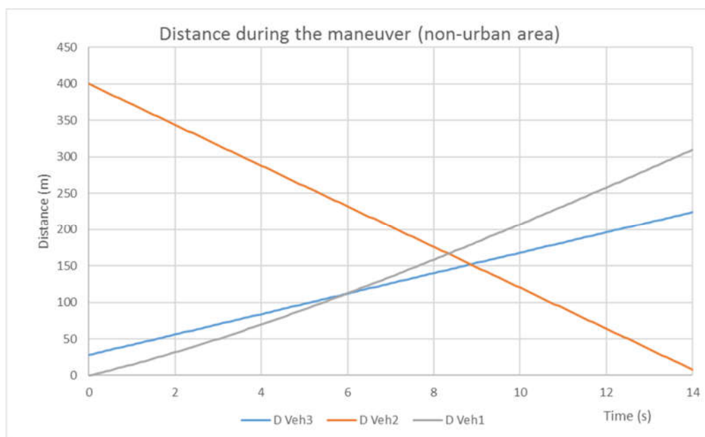
Figure B.5: Representation of the time – distance relation between the vehicles involved in the use case for non-urban area.
