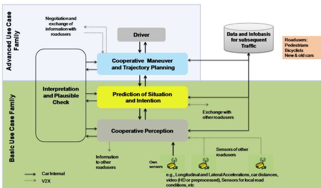
Figure B.2: Functional architecture.
