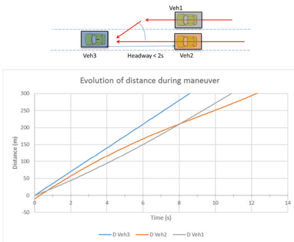
Figure B.3: Representation of the time – distance relation between the vehicles involved in the use case.
