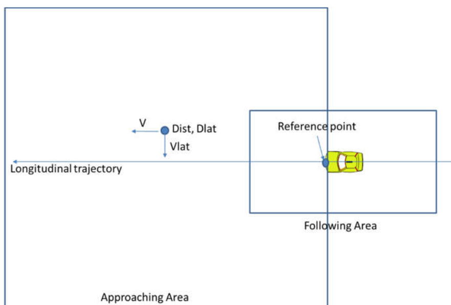
Figure 4.1: Detection/tracking areas in intersection situations.
