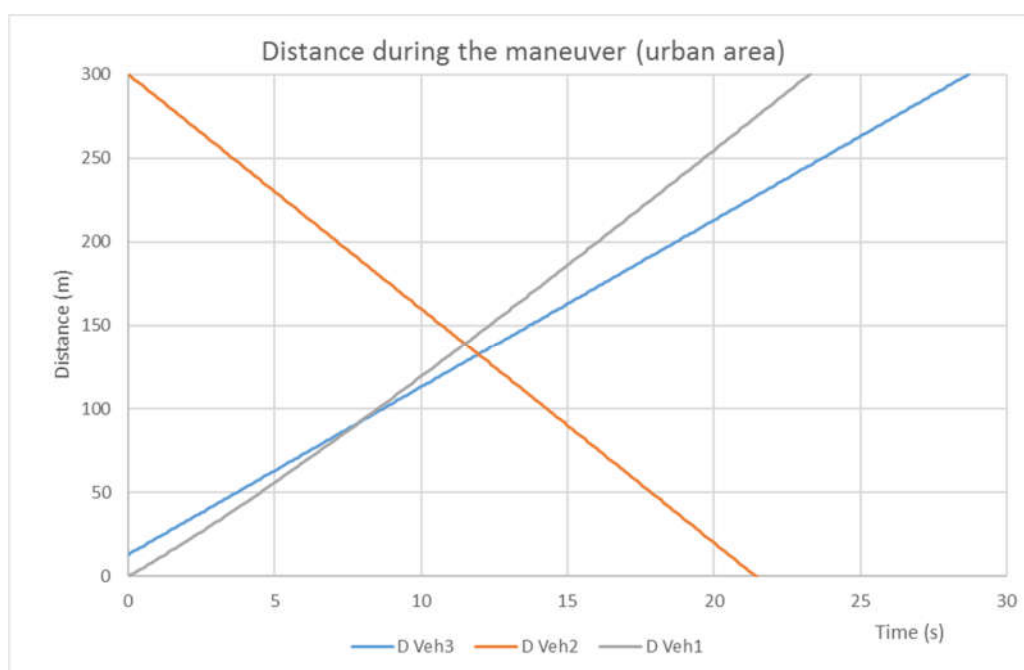
Figure B.6: Representation of the time – distance relation between the vehicles involved in the use case for urban area.
