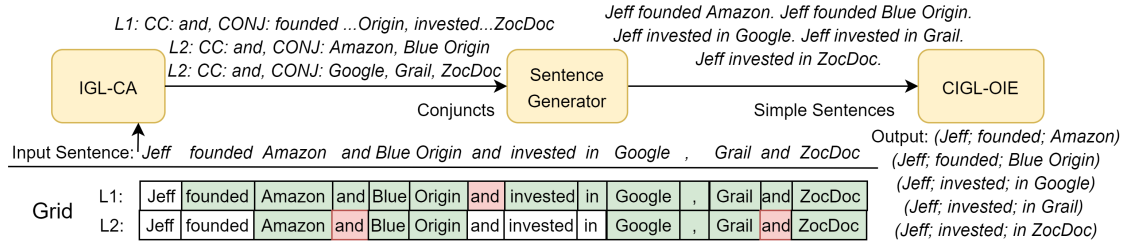
Figure 4: The final OpenIE system. IGL-CA identifies conjunct boundaries by labeling a 2-D grid. This generates simple sentences and CIGL-OIE emits the final extractions.
