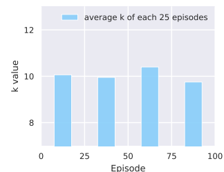
Figure 5: The k values selected by the adaptive coordinator of our LHUA agent
