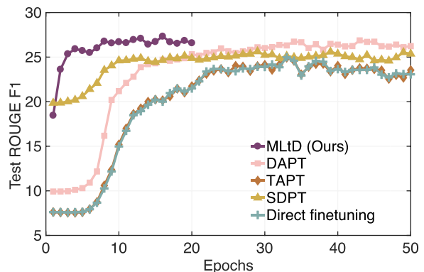
Figure 7: Convergence trajectories when finetuning BART upon applying each method on AdaptSum, using the Debate domain as an example.
