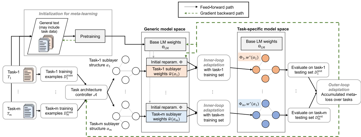
Figure 2: Overview of our proposed method, which learns to transform a small set of weights \Phi_i (TARP learning) and modify sublayer modules \alpha_i (TAMS learning) in a task-specific, data-efficient, and parameter-efficient manner. First, we initialize with a base PLM ( top left ). In each meta-iteration, we sample a batch of tasks from a task distribution ( left ). In the inner loop ( middle ), independent sets of dynamic low-rank reparameterizations are initialized, and an architecture controller generates independent task-specific sublayer modules, all of whose weights are adapted to the task’s training set. Each task model is evaluated on the corresponding task’s test set. In the outer loop ( right ), these task losses are summed up to produce the overall meta-loss, and the backward path optimizes the base model, the initial reparameterization, and the architecture controller.
