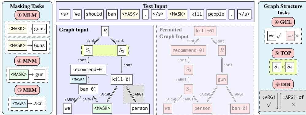
Figure 4: Pre-training Tasks for GreaseArG. MLM : Predict masked tokens in text input. MNM : Predict masked node attributes in graph input. MEM : Predict masked edge attributes in graph input. GCL : Predict whether a node belongs to the original or permuted graph input. TOP : Predict the relative order of consecutive link nodes. DIR : Predict the original edge direction. Note that the permuted graph input is only used by GCL.
