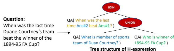
Figure 1: An illustration of H-expression.
