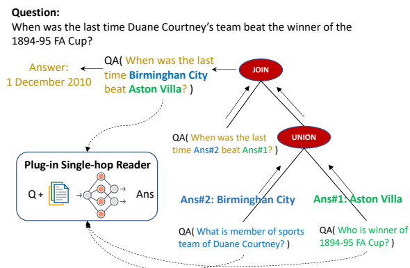
Figure 3: An overview of the H-executor. It involves execution of the question node and utilization of a plug-in neural reader to provide answer feedback for each question. Subsequently, the deterministic symbolic interpreter executes the expression to yield the final answer.
