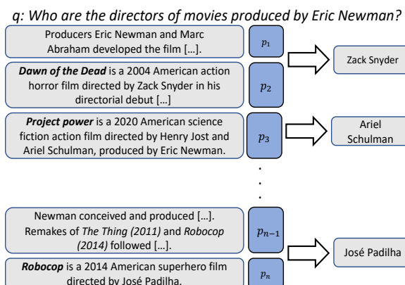
Figure 1: An example from QAMPARI with a generated question q , a subset of its evidence Wikipedia passages (left, p_i ) and their corresponding answer.
