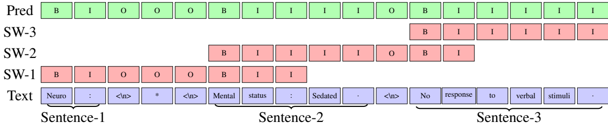
Figure 1: Sliding window algorithm for sentence segmentation. We segment the text using three sliding windows sequentially ( SW-1 , SW-2 , and SW-3 ). Each sliding window contains up to 8 tokens. The final sentence segmentation tags are at the top ( Pred ) of the diagram.
