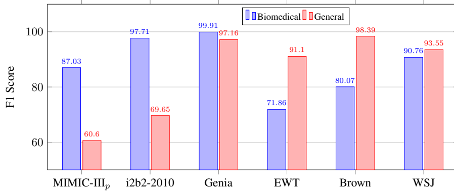
Figure 3: Cross-domain evaluation of our two Segementer-Domain models. The blue bars show the performance of the segmenter trained on a combination of three biomedical corpora, while the red bars represent the performance of the segmenter trained on a combination of three general domain corpora.
