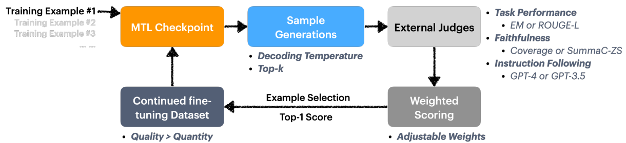
Figure 8: The illustration of our proposed method RESET. It samples generations from the initial vanilla multi-task learning (MTL) checkpoint with seen examples from instruction following and context-dependent datasets. For each example, it generates a set of possible responses with different decoding strategies. Generations are rated by external judges with a weighted scores of task performance, faithfulness and instruction following scores. Then, the top rated generations will be collected to further fine-tune the initial model.
