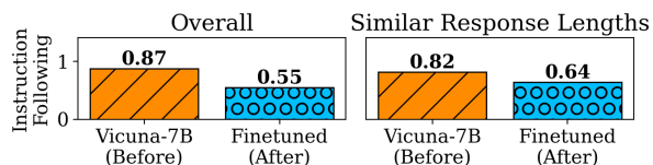
Figure 7: Instruction following scores for 1,000 randomly selected examples from Alpaca-15K (left), and for filtered examples with similar generation lengths (maximally 10 tokens longer) before and after fine-tuning with context-dependent datasets (right).
