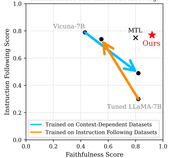
Figure 1: Faithfulness scores on context-dependent tasks (QA and summarization) decrease when we fine-tune grounded LLaMA-7B checkpoint with instruction following datasets (orange), and instruction following scores (assessed by GPT-4) decrease when we fine-tune Vicuna-7B with context-dependent tasks (blue). Our method, RESET surpasses the vanilla MTL with data mixing, approaching the North Star (upper right corner).
