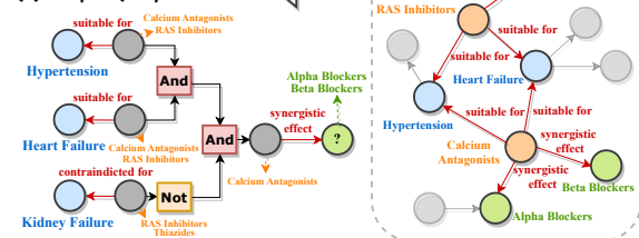
Figure 1: An example of KBQA task to answer a natural language question by converting the question to a graph query which can be executed over Knowledge Base.
