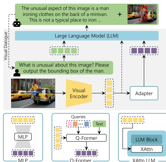
Figure 1: General architecture of Multimodal Large Language Models (MLLMs), composed of a visual encoder, a language model, and an adapter module that connects visual inputs to the textual space.
