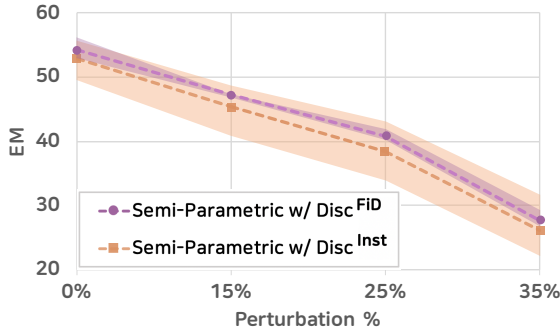
Figure 3: Comparison of GPT-3.5’s stability for each discriminator setting. The shaded area represents the variance computed between the best and worst EM.
