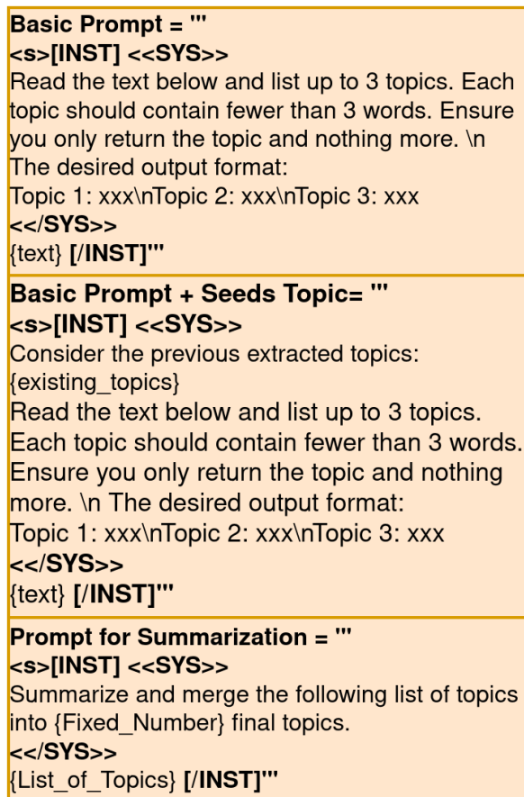
Figure 1: Example prompts for LLaMA. Text enclosed by the special tokens ‘<<SYS>>’ is designated as a system prompt.
