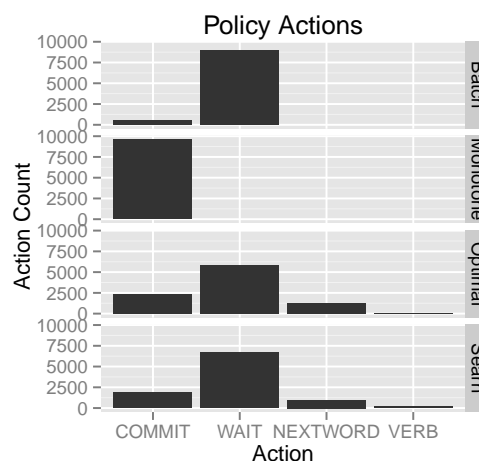
Figure 5: Histogram of actions taken by the policies.
