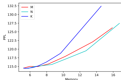
Figure 2: Influence of M, N, K for PTB-small.
