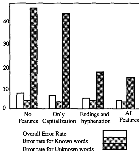
Figure 1: Decreasing error rate with use of word features
