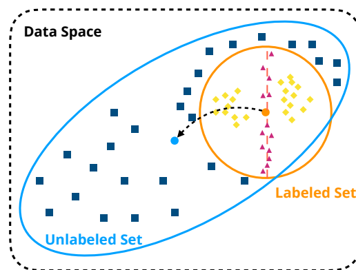
Figure 1: Illustration of sample-selection issues in co-training methods. (1) Randomly sampled unlabeled examples ( \square ) will result in high sampling bias, which will cause bias shift towards the unlabeled dataset ( \leftarrow ). (2) High-confidence examples ( \diamond ) will contribute little during the model training, especially for discriminating the boundary examples ( \triangle ), resulting in myopic trained models.
