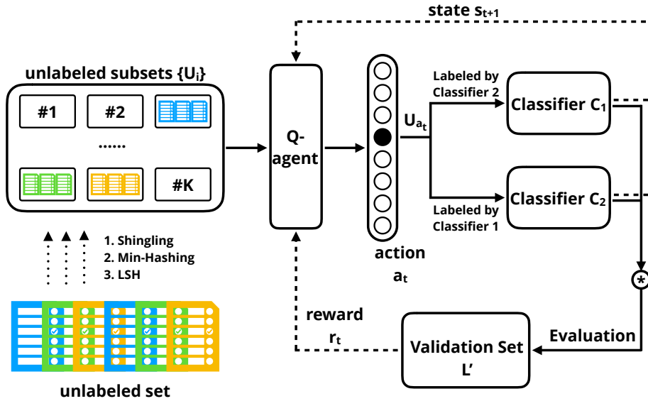
Figure 2: The Reinforced Co-Training framework.
