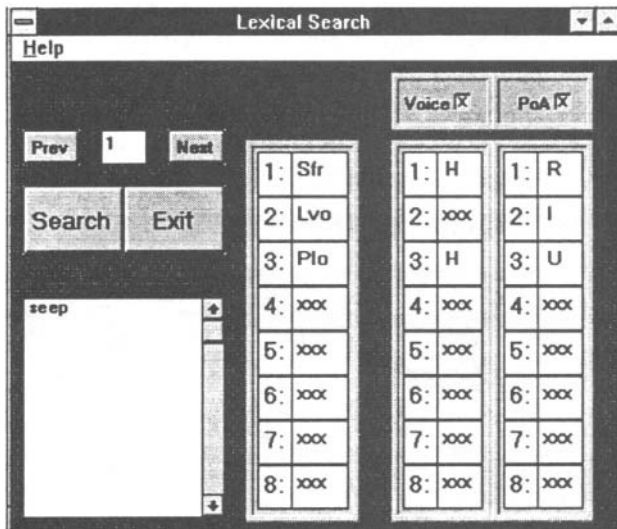
Figure 4. Lexical search screen for a common manner class sequence (Stage 3)
