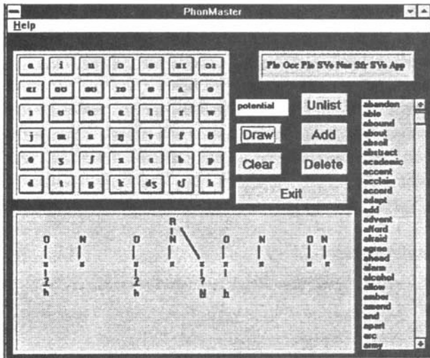
Figure 2. Representation of potential after Stage 1
