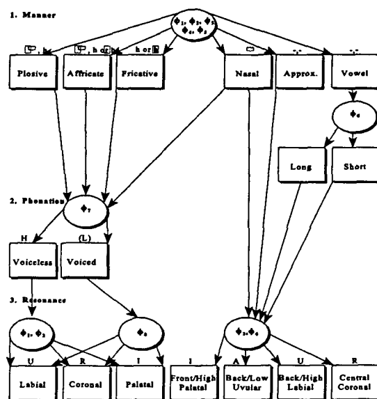
Figure 1. Stagewise cue invocation strategy
