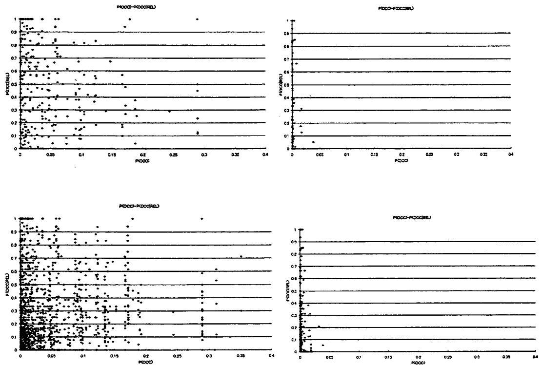
Figure 1: p(\text{occ}|\text{rel}) as function of p(\text{occ})
