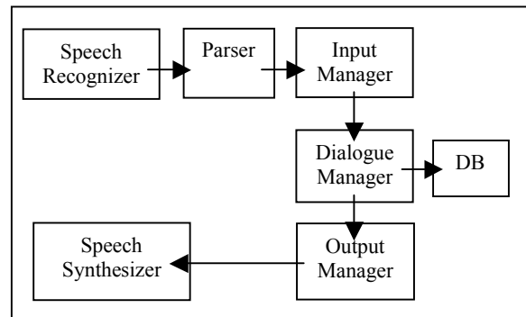
Figure 5. A more typical dialogue system architecture, with the side effects executed separately from the spoken output.
