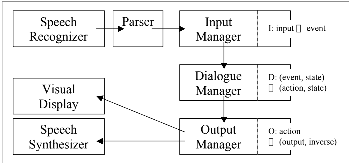
Figure 4. Checklist dialogue system architecture.
