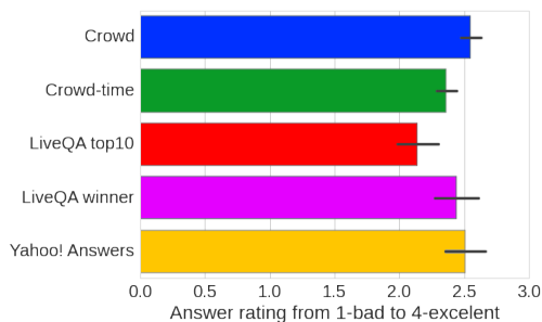
Figure 6: Average scores of different types of answers to Yahoo! Answers questions
