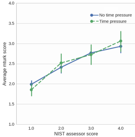
Figure 3: Correlation between NIST assessor scores and crowdsourced ratings with and without time limit on the work time
