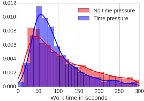
Figure 5: Distribution of answering times for experiments with and without time pressure
