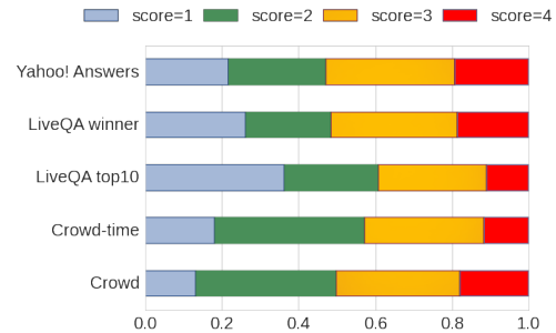
Figure 7: Distribution of scores for different types of answers to Yahoo! Answers questions
