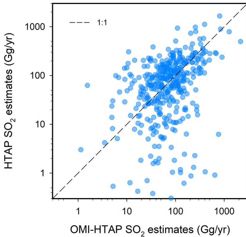
Figure S1: Comparison of 2010 OMI-HTAP and HTAP SO 2 emissions for OMI-detected sources. Emissions for individual sources are calculated by summing up SO 2 emissions of each grid cells in the fitting domain (see Sect.2.1) from two inventories.
