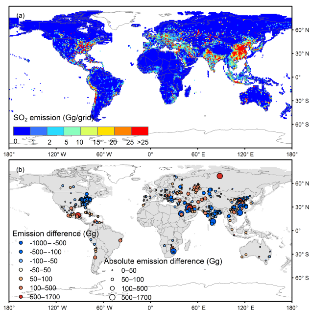
Figure 2. (a) Map for SO 2 emissions in the OMI-HTAP inventory, 2010. Emissions are regridded at the resolution of 1^\circ \times 1^\circ for illustration. The unit is Gg-SO 2 per grid cell. The grid cells without SO 2 emissions are color coded with white. (b) The differences in emissions for individual OMI-detected sources between the OMI-HTAP and the HTAP inventory, 2010. Emissions for individual sources are calculated by summing up SO 2 emissions of each grid cells in the fitting domain (see Sect. 2.1). SO 2 emissions derived from the HTAP inventory are subtracted from those derived from the OMI-HTAP inventory to calculate the differences. The grid cells without emissions changes are color coded with grey. The unit is Gg-SO 2 per year.
