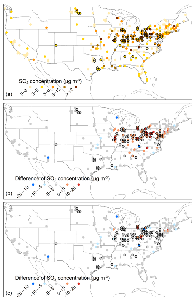
Figure 5. Annual averaged SO 2 surface concentrations from AQS measurements in 2010 (a) and their differences between the modeled SO 2 using the HTAP (b) and the OMI-HTAP inventory, 2010 (c). AQS measurements are subtracted from the modeled SO 2 to derive the differences. The outline of circles corresponding to the grid cells with differences in emissions between the HTAP and the OMI-HTAP inventories is highlighted in black.
