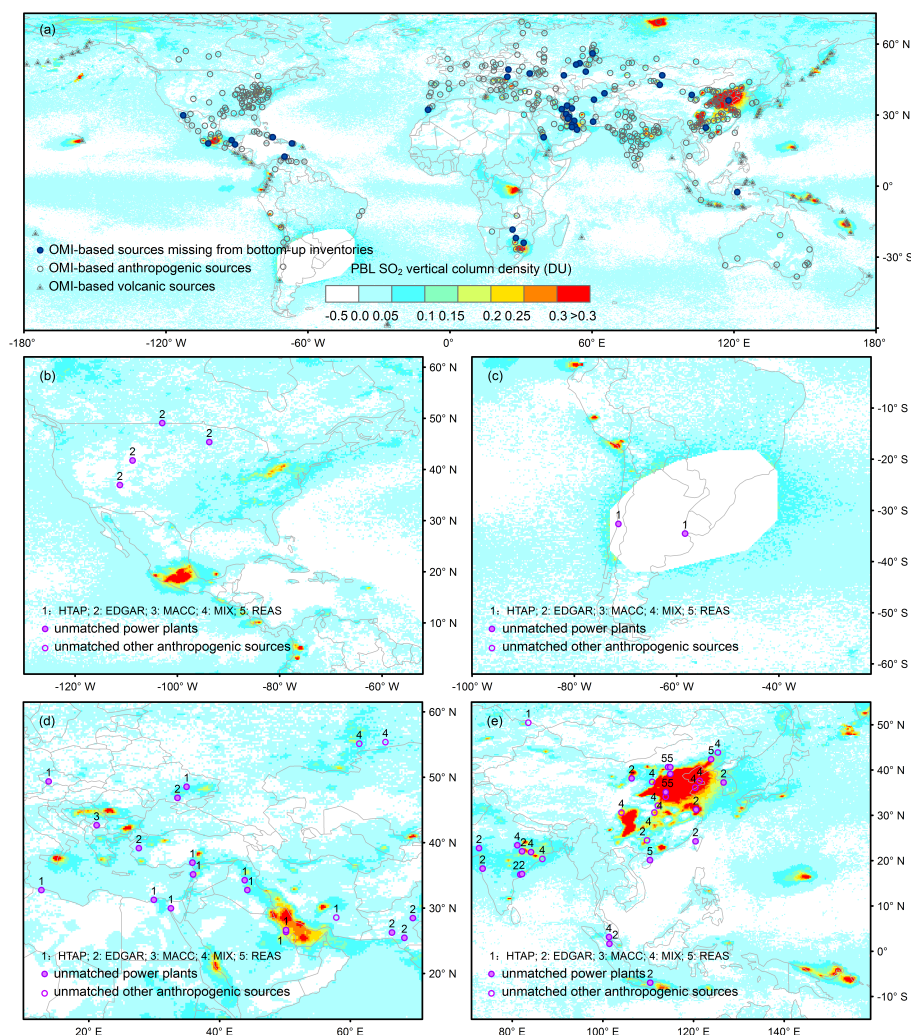
Figure 8. (a) Geographic distribution of SO 2 sources in the OMI-based emission catalogue (Fioletov et al., 2016). SO 2 sources identified that were found to be missing from bottom-up inventories are in blue. Locations of large sources indicated by bottom-up inventories but not detected by OMI (unmatched) over (b) North America, (c) South America, (d) Europe, and (e) Asia. The background is the global mean SO 2 distribution (in DU) map for 2005–2014. The area affected by the South Atlantic Anomaly is shown as a white oval.
