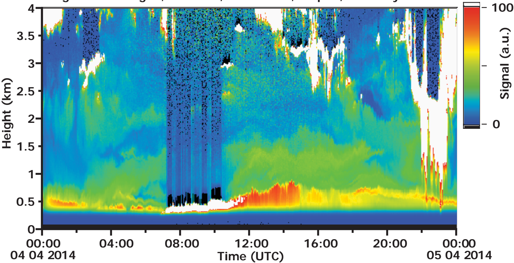
Range-corrected signal, 1064 nm, Ceilometer, Melpitz, Germany
