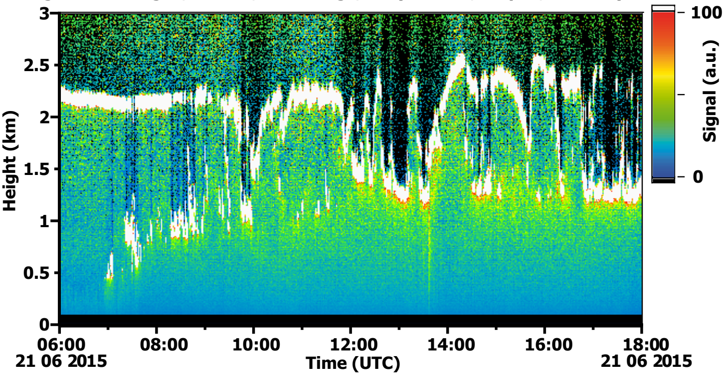
Range-corrected signal, 532 nm, near-range, PollyXT lidar, Melpitz, Germany
