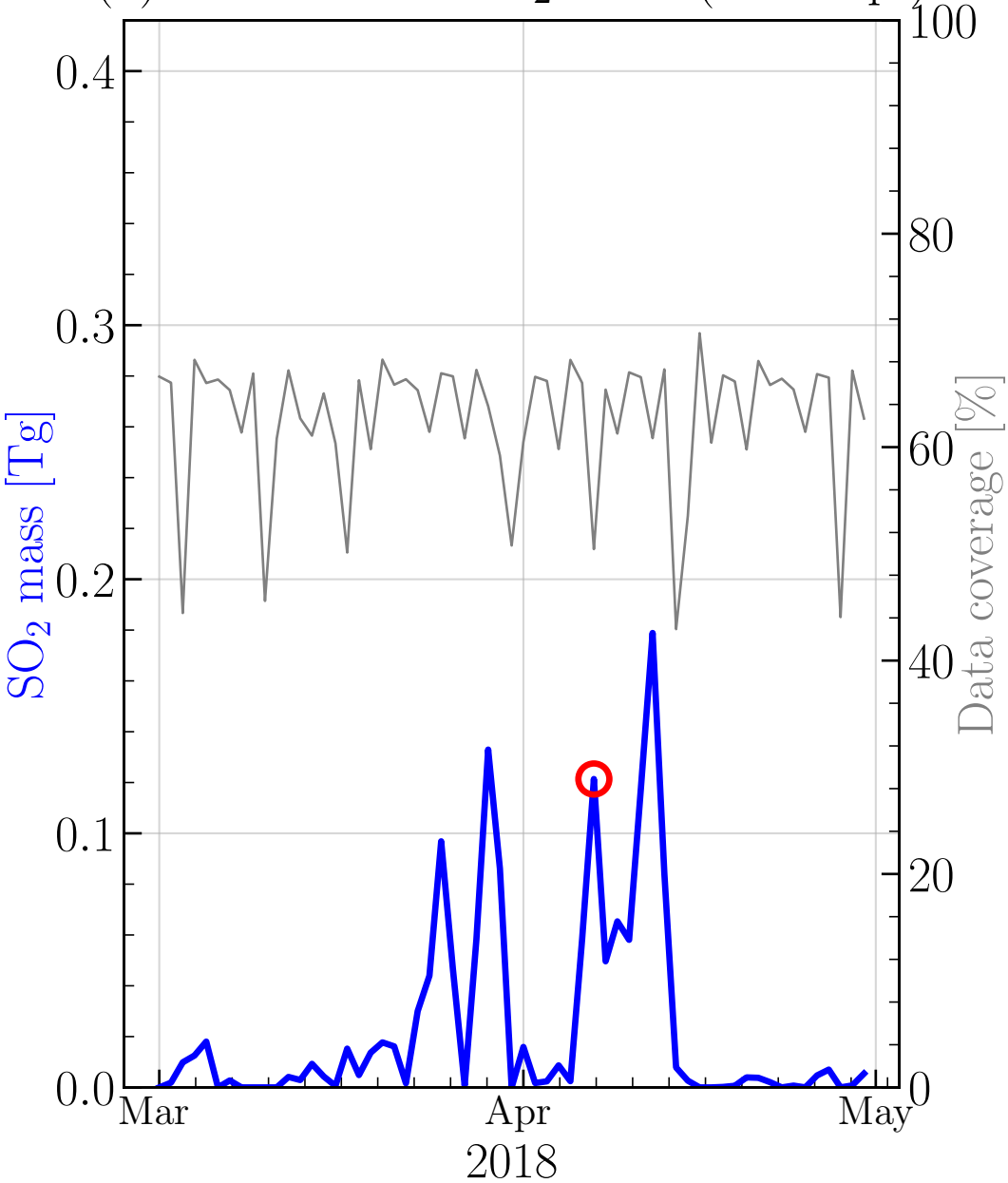
(a) OMI OMPS SO 2 mass (1st erup.)
