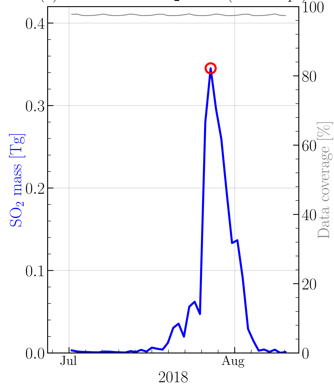
(c) TROPOMI SO 2 mass (2nd erup.)
