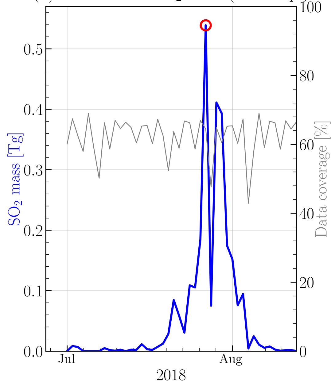
(b) OMI OMPS SO 2 mass (2nd erup.)
