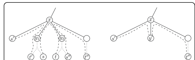
Figure 1 Applicability of reduction. Left: Illustration of the structure for a deepest least common ancestor x of the pairs as described in the proof of Lemma 1. The dashed lines represent the paths between the endpoints of a pair. If [s, t] is in conflict with two other pairs, then these pairs must be conflicting with [s, t] in the edges \{x, y_1\} and \{x, y_2\} since x a deepest least common ancestor. Right: Illustration of the replacement of the subtrees rooted at y_1 and y_2 by a single vertex y . Note that (s', y) and (y, t'') are in conflict.
