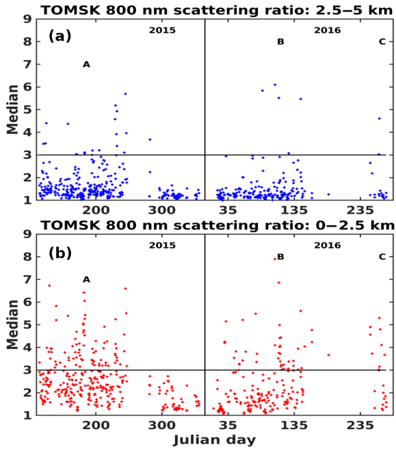
Figure 7. Time evolution from April 2015 to September 2016 of the median of the 800 nm Tomsk lidar backscatter ratio for two altitude ranges: 0–2.5 km (b) and 2.5–5 km (a). A, B and C are the cases analysed in Sect. 5.
