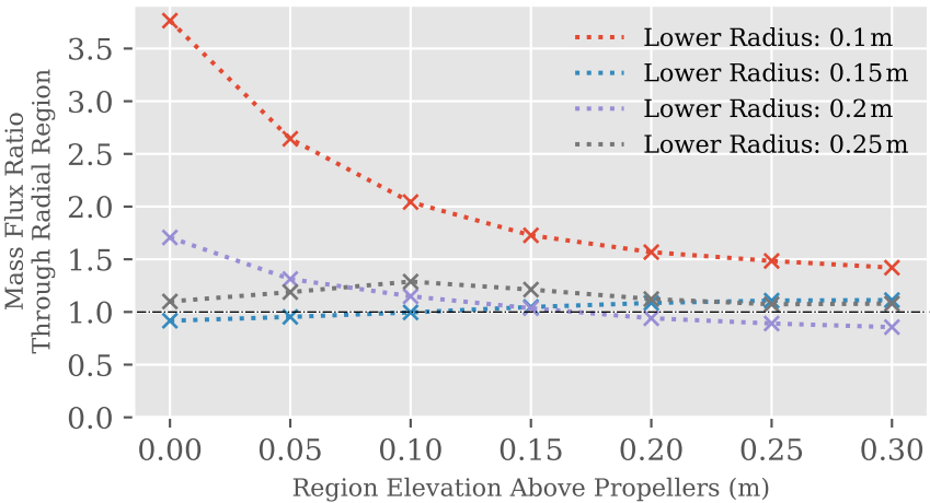
Mass Flux Ratio Through Radial Regions Against Height
