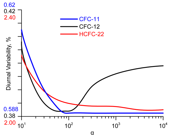
Figure 3. Dependence of the TCs intraday variability in the regularization parameter \alpha .
