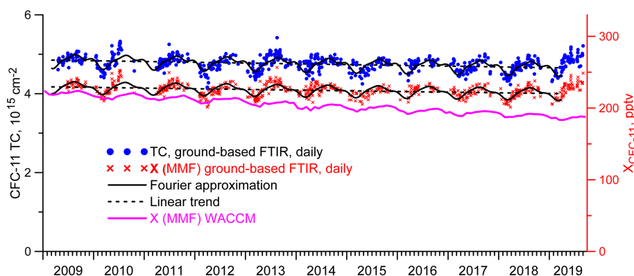
Figure 4. Daily mean TCs and X gas of CFC-11. The T–Ph parameter \alpha = 85 .
