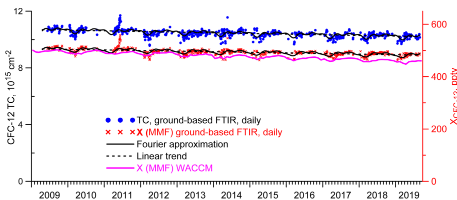
Figure 5. Daily mean TCs and X_{\text{gas}} of CFC-12. Filtered results of the T–Ph parameter \alpha = 85 .
