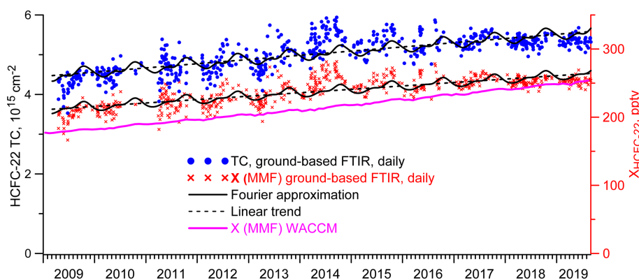
Figure 6. Daily mean TCs and X_{\text{gas}} of HCFC-22. Filtered results of the T–Ph parameter \alpha = 3 \times 10^3 .
