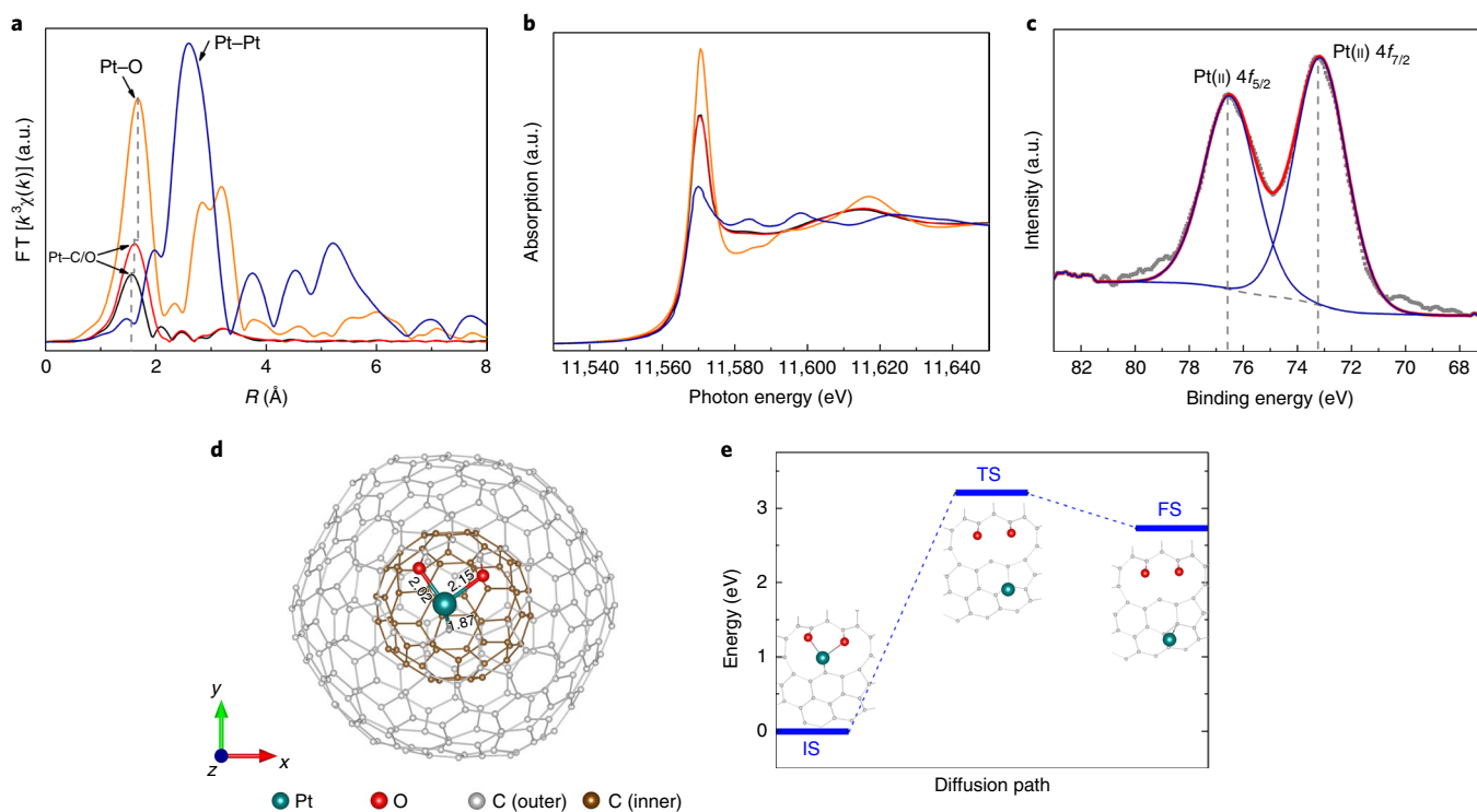
Fig. 2 | Structural identification of Pt single atom in Pt 1 /OLC catalyst. a, b , The Pt L 3 edge FT-EXAFS spectra of Pt 1 /OLC (red), along with PtO 2 (yellow), Pt foil (blue) and the Pt ligands/OLC (black) (without O 3 exposure to remove their ligands in MeCpPtMe 3 precursors) for comparison ( a ) and the corresponding normalized XANES spectra ( b ). c , High-resolution XPS Pt 4f spectrum of Pt 1 /OLC, where it is fitted by fixing the spin-orbit splitting of 3.3 eV and area ratio of 4:3 for a doublet pair (4f 7/2 and 4f 5/2 ). d , The optimized atomic model of PtO 2 C 295 , which exhibits Pt–O bonding in accordance with the experiments, where the grey and brown balls represent the carbon atoms in the outer/inner shell of fullerene-like structure. e , The lowest diffusion barrier (most probable diffusion path) of a Pt atom on PtO 2 C 295 is as high as 3.2 eV, which demonstrates the stability of Pt anchoring. IS, initial state; TS, transition state; FS, final state. a.u., arbitrary units.
