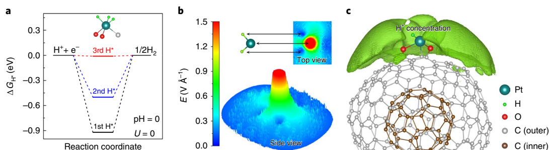
Fig. 4 | Theoretical investigation of the HER using the Pt t /OLC catalyst. a , Calculated free-energy diagram of the HER at the equilibrium potential with pH = 0 and assuming that Pt is the active site. The inset shows the model of H adsorbed on the Pt site, where light green, green, red and grey balls represent, respectively, hydrogen, platinum, oxygen and carbon atoms. b , The map of the electric field shows a localized electric field of the H 2 Pt t /OLC system at the tip-like Pt site with an equilibrium potential. c , Based on the Gouy-Chapman-Stern model, a high concentration of protons (>1.99 mol l -1 ) is distributed around the Pt site (represented by the green shape), which is induced by the local electric field at the Pt site. The grey carbon atoms consist of the outer fullerene-like structure of OLC, whereas the brown carbon atoms represent the inner shell.
