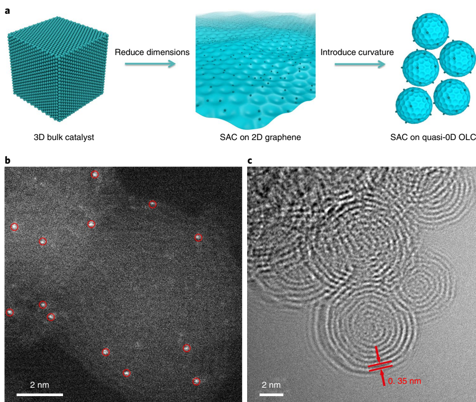
Fig. 1 | Rational design of the Pt t /OLC catalyst via reducing the dimensions and introducing curvature. a , The schematic illustrates the approach taken in this work, whereby catalytically active particles were reduced in size to a single-atom form and the dimensionality of the catalyst support was reduced by using quasi-0D OLCs. b , The HAADF-STEM image of Pt t /OLC clearly displays the Pt single atoms (highlighted by red circles) randomly dispersed on the OLC supports. c , Transmission electron microscopy image of Pt t /OLC shows a multishell fullerene structure with a layer distance of 0.35 nm.
