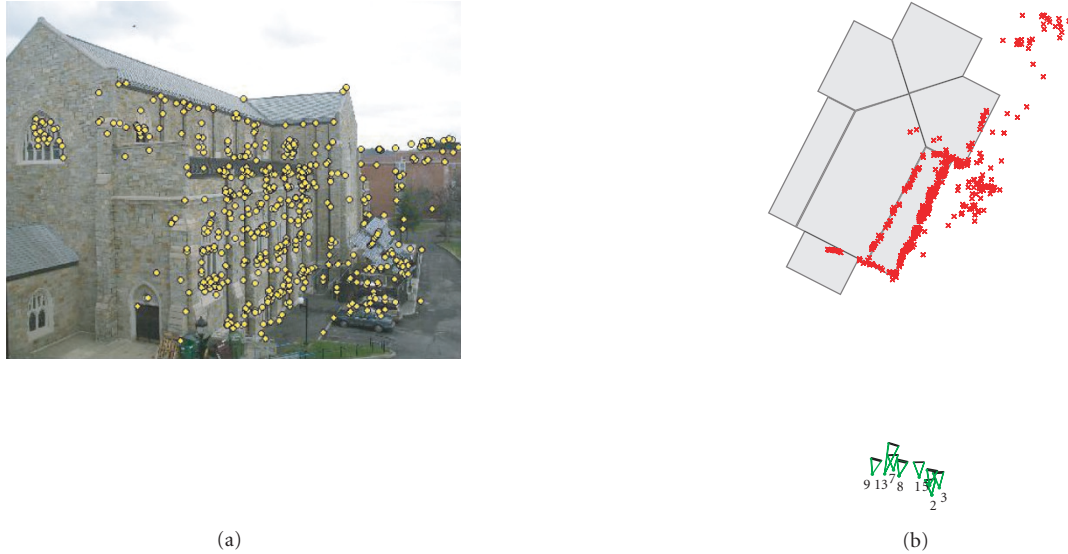
FIGURE 8: Camera calibration results for a prominent building in the scene. (a) Original image 2, with detected feature points overlaid. (b) The 3D reconstruction of the corresponding scene points and several cameras obtained by the distributed calibration algorithm, seen from an overhead view, with building shape manually overlaid. Parallel and perpendicular building faces can be seen to be correct. Focal lengths have been exaggerated to show camera viewing angles. This is only a subset of the entire calibrated camera network.
