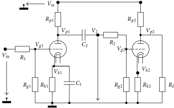
FIGURE 3: Circuit schematic of the first block of the guitar preamp.
