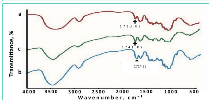
Figure 5: FTIR spectra of a) Bleached jute fiber, b) MVK-modified fiber and c) VA-modified jute fiber.
