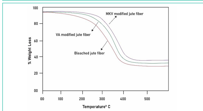
Figure 7: TGA thermograph of bleached, VA and MVK-modified jute fibers.
