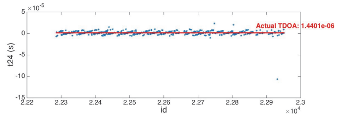
Fig. 7. TDOA extraction
