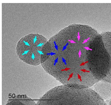
6(c): Beechwood soot
