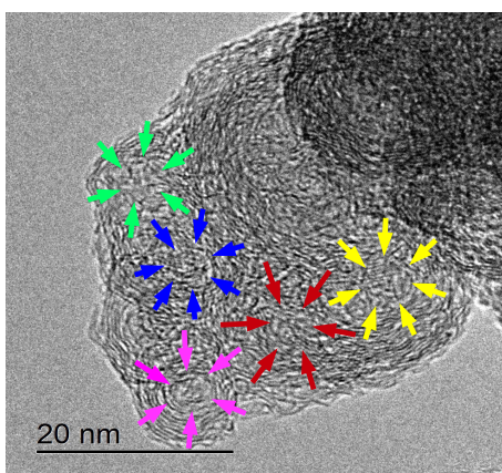
5(d): Activated tire carbon black
