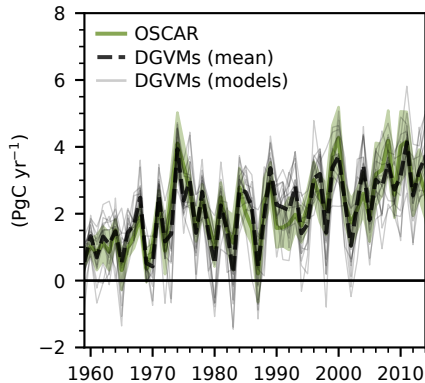
(b) Land sink without LULCC
