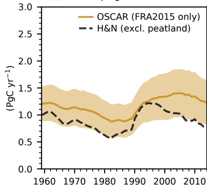
(f) Bookkeeping LULCC emissions
