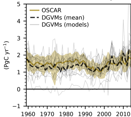
(c) LULCC emissions including LASC
