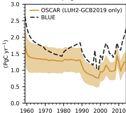
(e) Bookkeeping LULCC emissions
